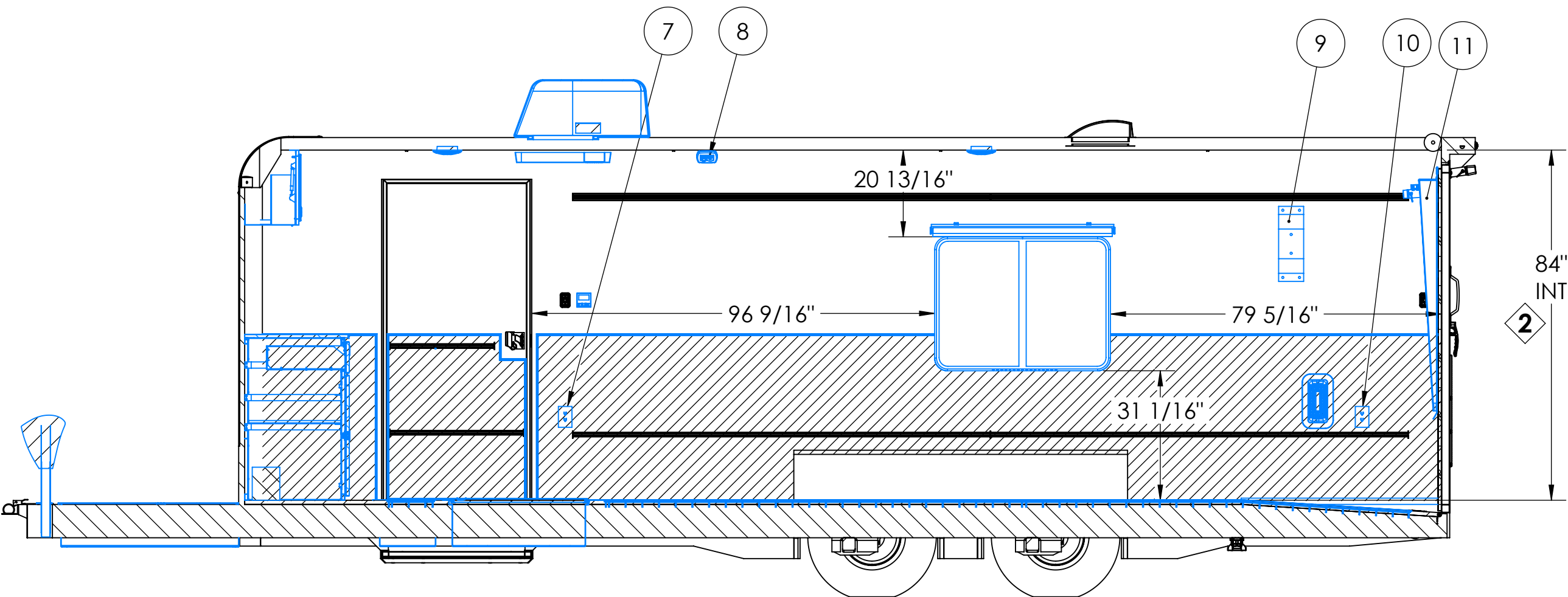
SECTION C-C SCALE 1 : 28
